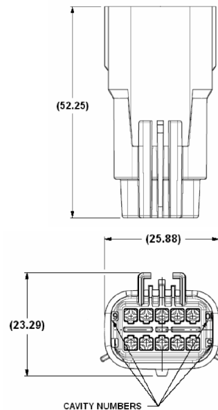
MALE
