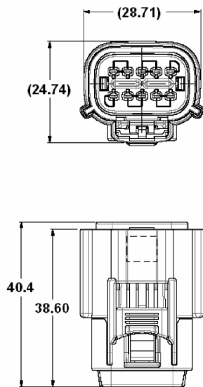
FEMALE
